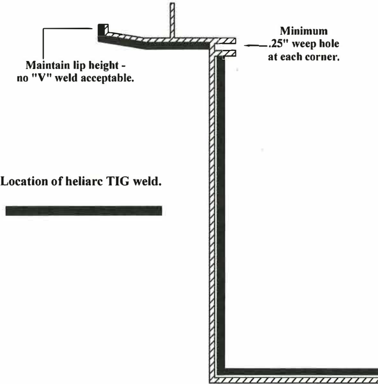
Detail #3 Aluminum Shape Weld Detail Tower Part #10947
